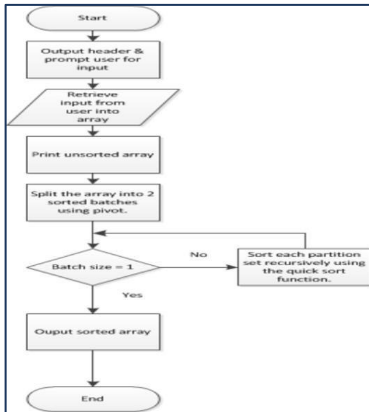
Figure 7.1: Flowchart of Quick Sort Partition and Recursive Execution
