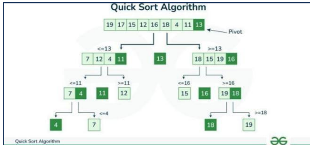
Figure 4.1: Divide and Conquer Partitioning Tree of Quick Sort Algorithm
